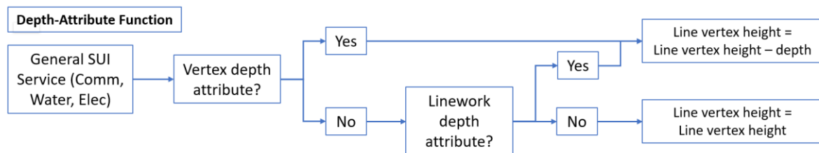
Figure 1: The Depth-Attribute Function. Program flow for typical services.
